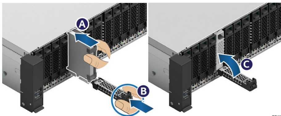
Figure 60. 7-mm Drive Insertion into 2.5" Drive Bay
