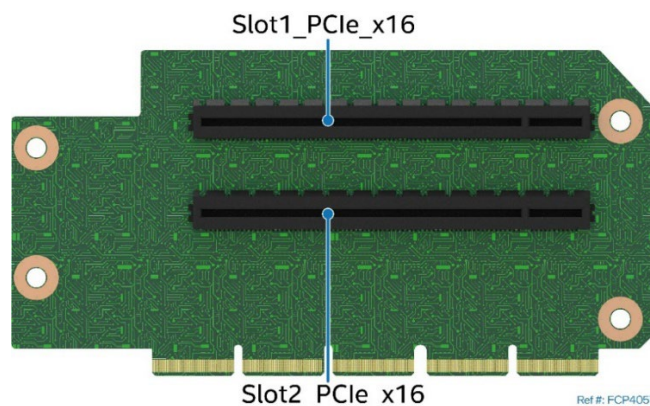
Figure 48. Two-Slot PCIe* Riser Card for Riser Slot #1
