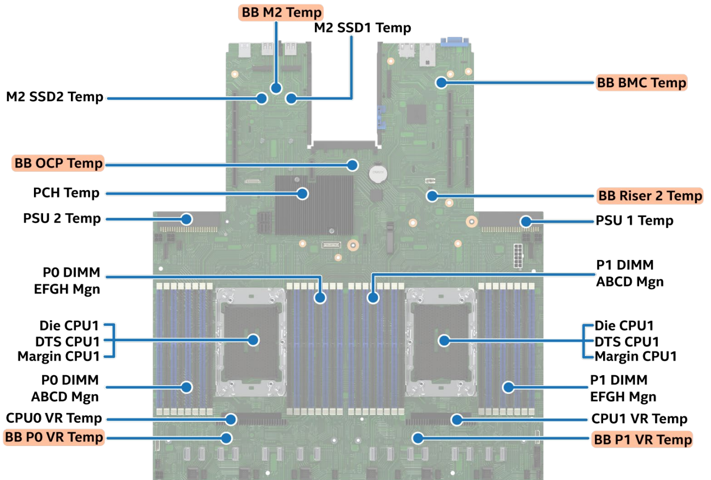
Figure 105. Server Board Sensor Map
