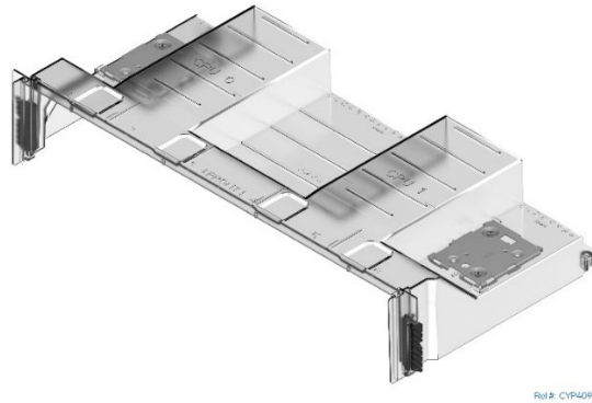
Figure 37. Standard Air Duct for 2U Height Processor Heat Sinks
