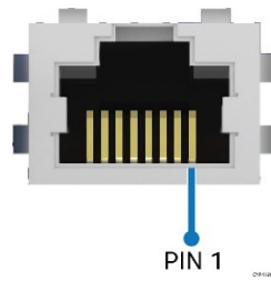
Figure 98. RJ45 Serial Port A Connector Pin Orientation
