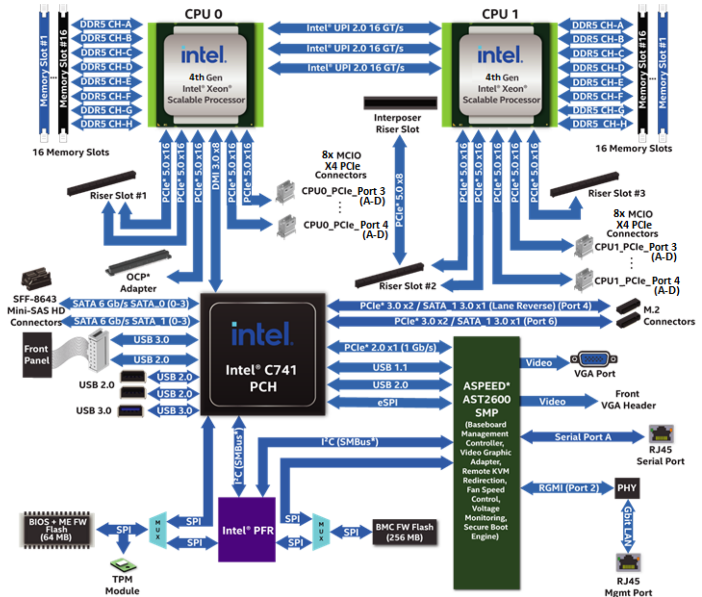
Figure 13. Intel® Server Board M50FCP2SBSTD Architectural Block Diagram
