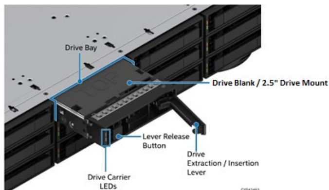
Figure 63. 3.5" Drive Bay Components
