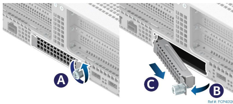
Figure 57. OCP* Adapter Bay Filler Removal
