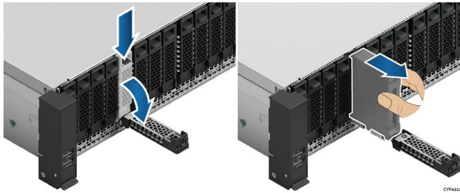
Figure 61. 7-mm Drive Removal from 2.5" Drive Bay
