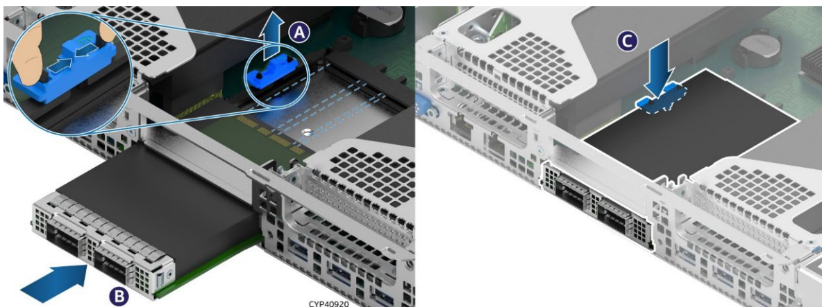
Figure 43. OCP* Adapter with Internal Lock Installation
