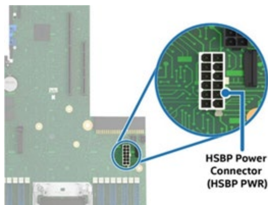
Figure 55. Server Board HSBP Power Connector
