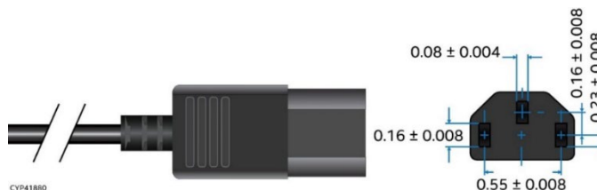
Figure 25. AC Power Cord Specification
