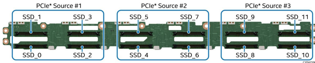
Figure 65. 12 x 2.5" SAS/SATA/NVMe* Hot Swap Backplane – Front Side
