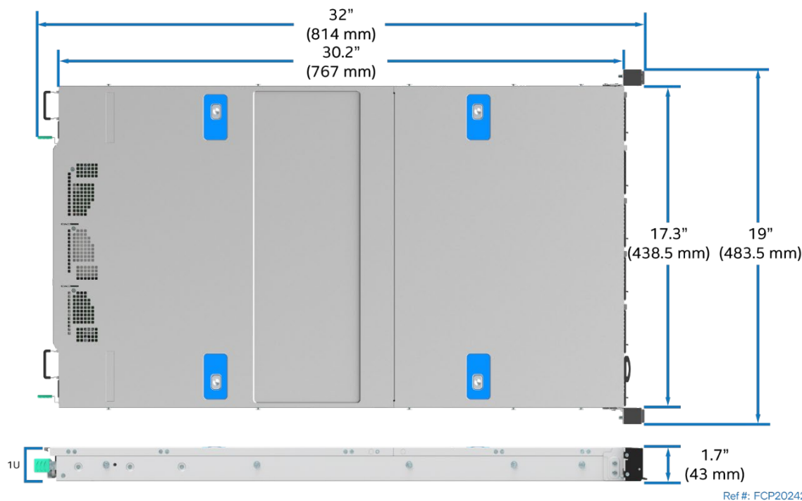
Figure 12. System Dimensions
