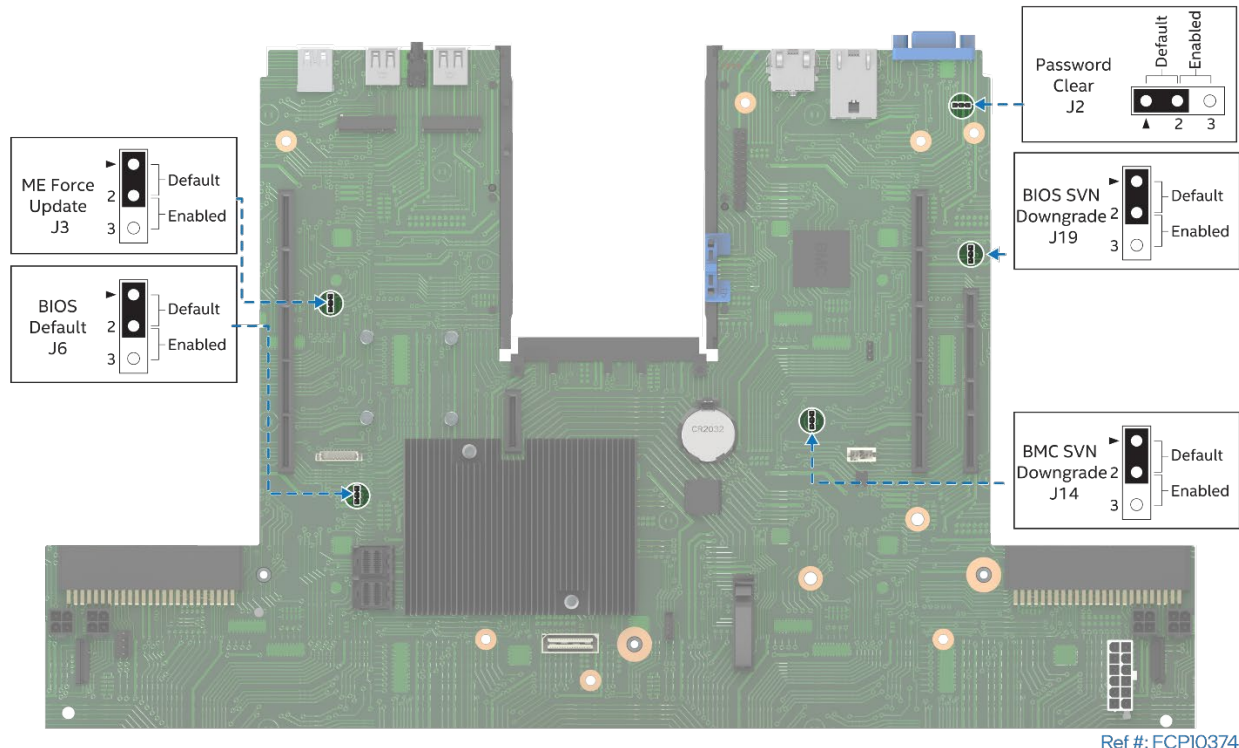
Figure 11. System Configuration and Recovery Jumpers
