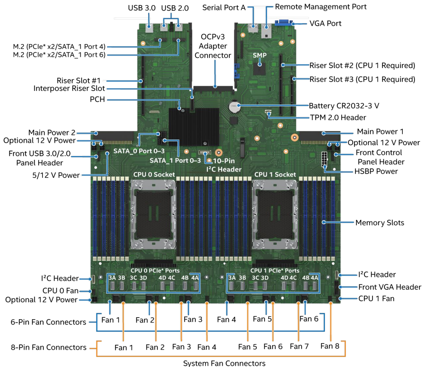
Figure 8. Intel® Server Board M50FCP2SBSTD Component / Feature Identification
