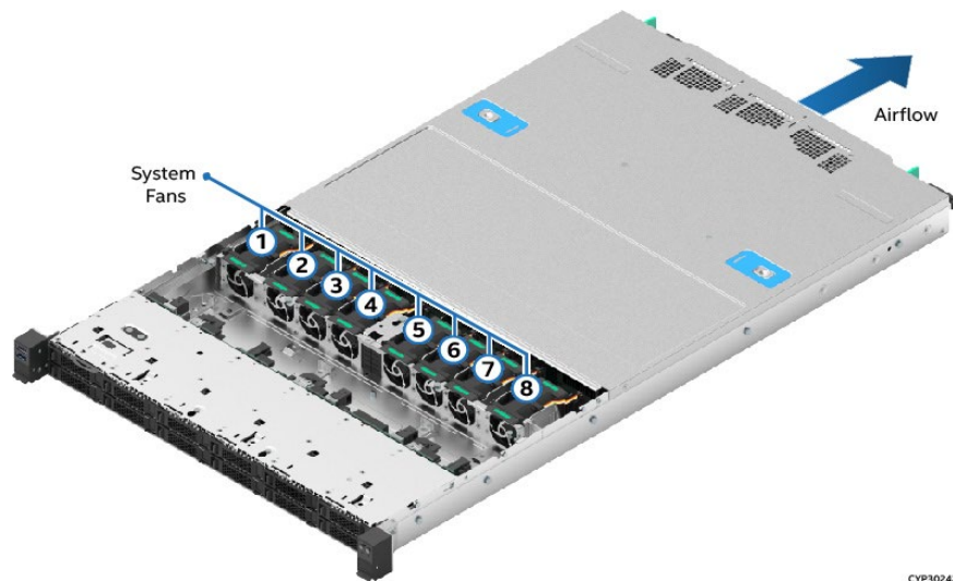
Figure 26. System Airflow and Fan Identification
