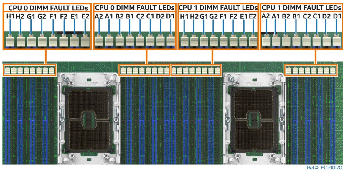
Figure 10. Intel® Light-Guided Diagnostics – Memory Fault LEDs
