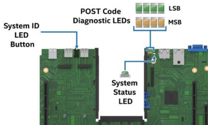
Figure 75. Exploded View of POST Code Diagnostic, System ID, and System Status LEDs
