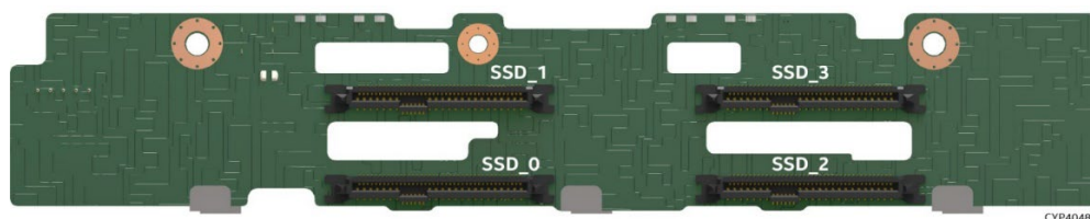
Figure 56. 4 x 2.5" SAS/SATA/NVMe* Hot Swap Backplane – Front Side
