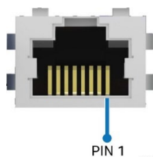
Figure 73. RJ45 Serial Port A Pin Orientation
