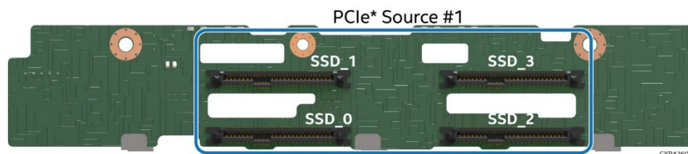
Figure 63. 4 x 2.5" SAS/SATA/NVMe* Hot Swap Backplane – Front side
