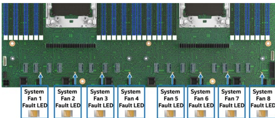
Figure 79. System Fan Fault LEDs
