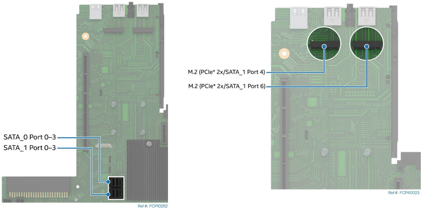
Figure 67. Onboard SATA Cable Connectors and M.2 SSD Connectors
