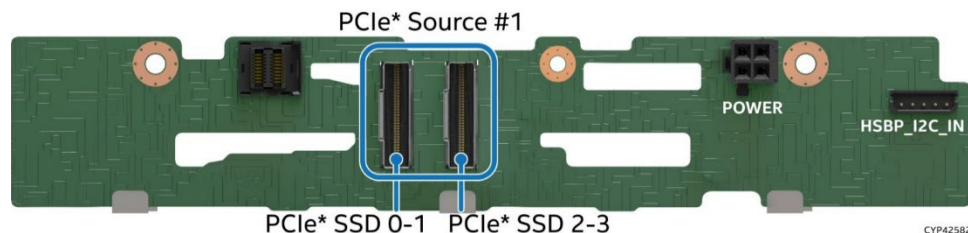
Figure 64. 4 x 2.5" SAS/SATA/NVMe* Hot Swap Backplane – Back Side
