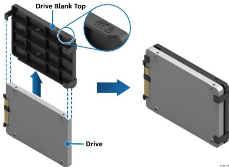
Figure 49. 7mm SSD Support
