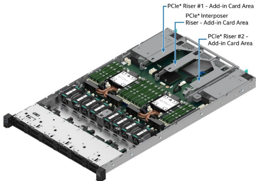
Figure 31. PCIe* Riser Card Slot Identification
