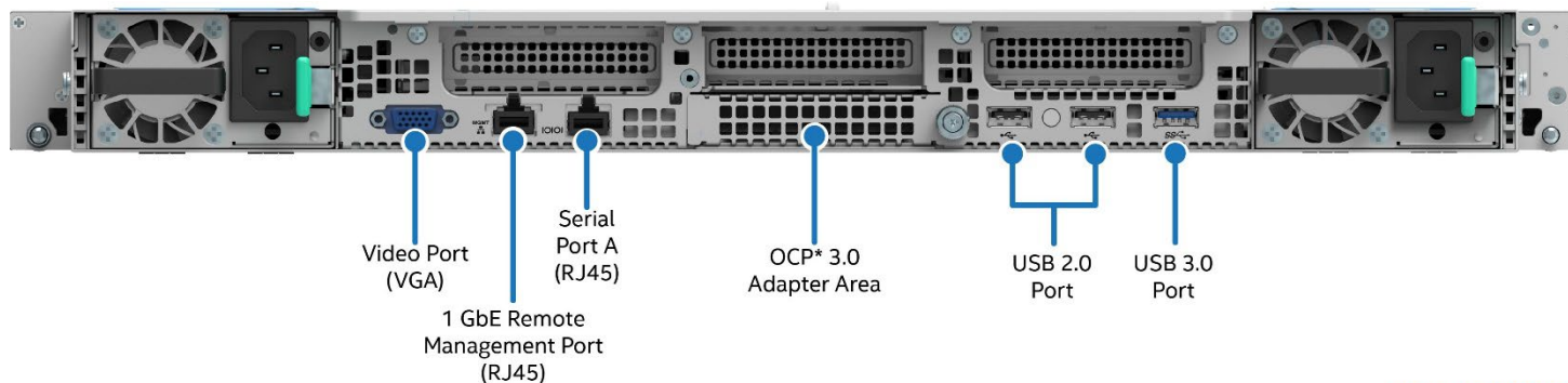
Figure 70. Rear I/O Features
