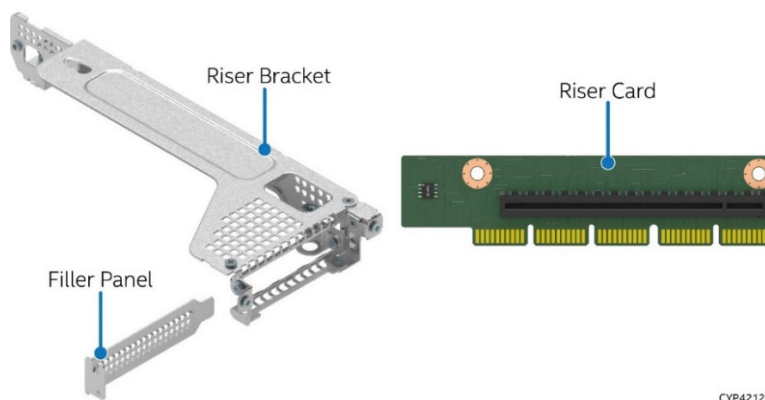
Figure 32. Riser Card Assembly Components
