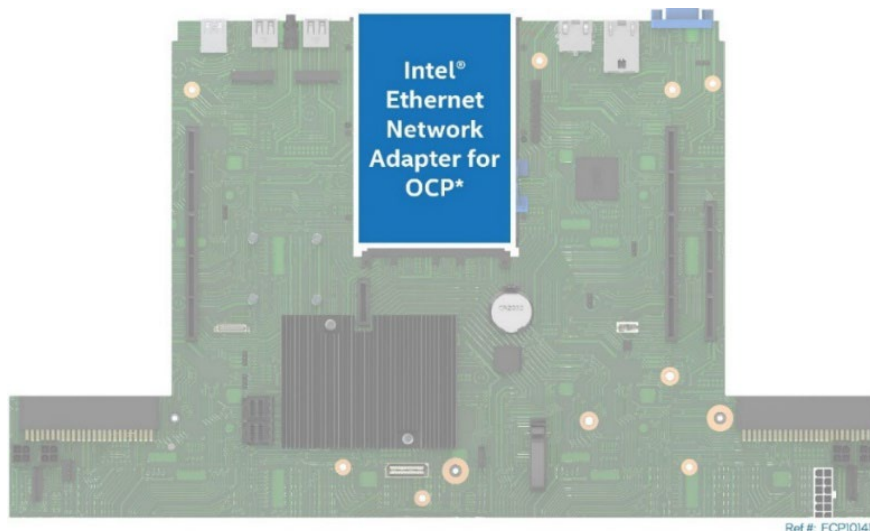
Figure 40. Intel® Ethernet Network Adapter for OCP* Placement
