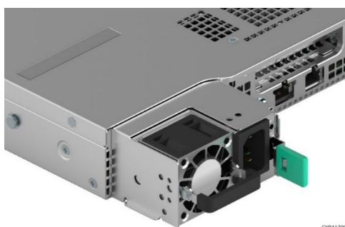
Figure 22. Power Supply Module Partially Out of Chassis
