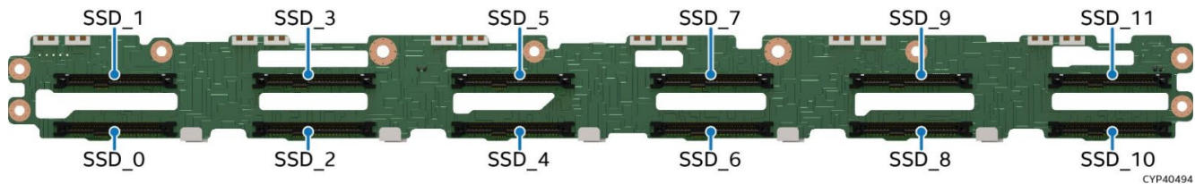
Figure 58. 12 x 2.5" SAS/SATA/NVMe* Hot Swap Backplane – Front Side
