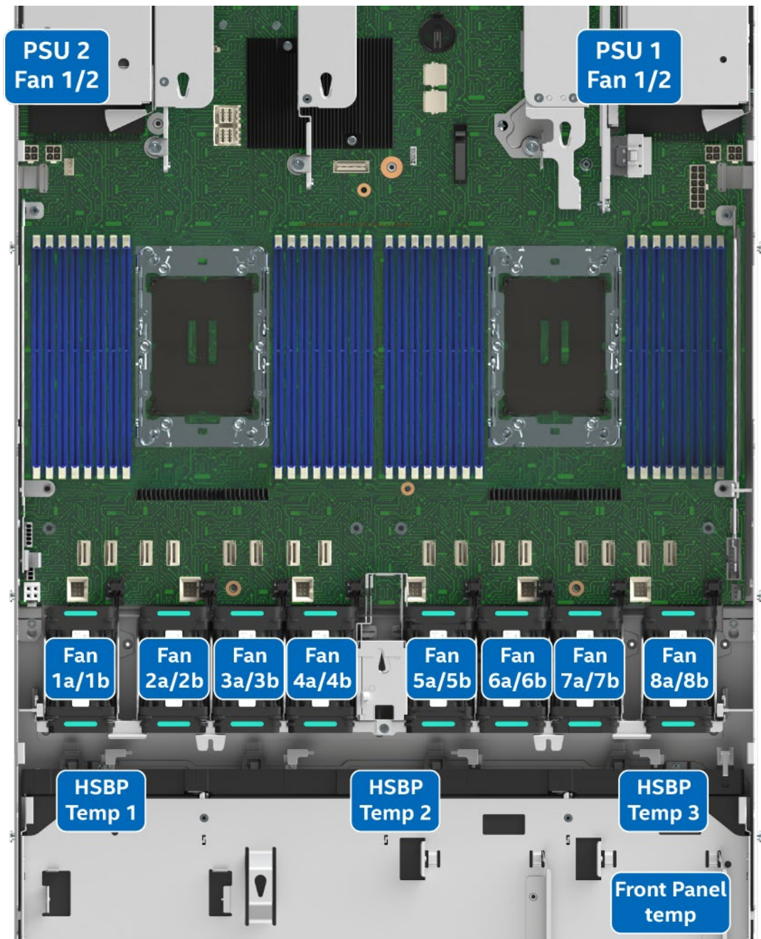
Figure 81. Server System Sensor Map
