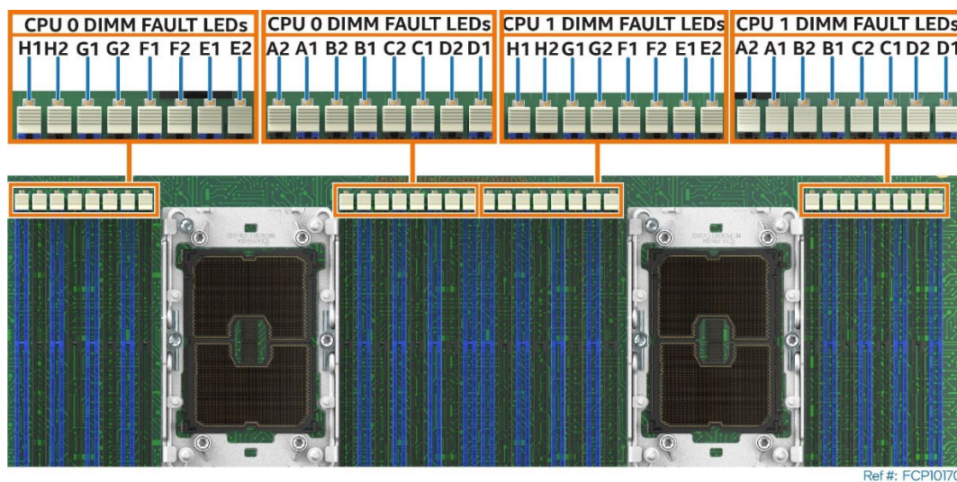
Figure 78. Memory Fault LED Location
