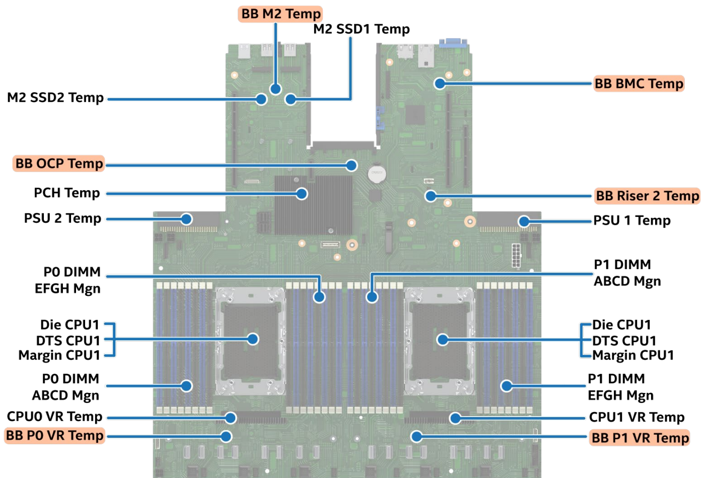
Figure 80. Server Board Sensor Map
