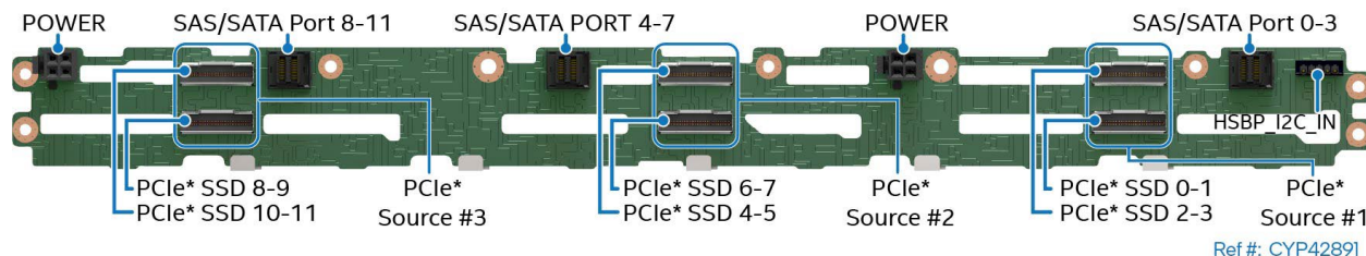
Figure 66. 12 x 2.5" SAS/SATA/NVMe* Hot Swap Backplane – Back Side
