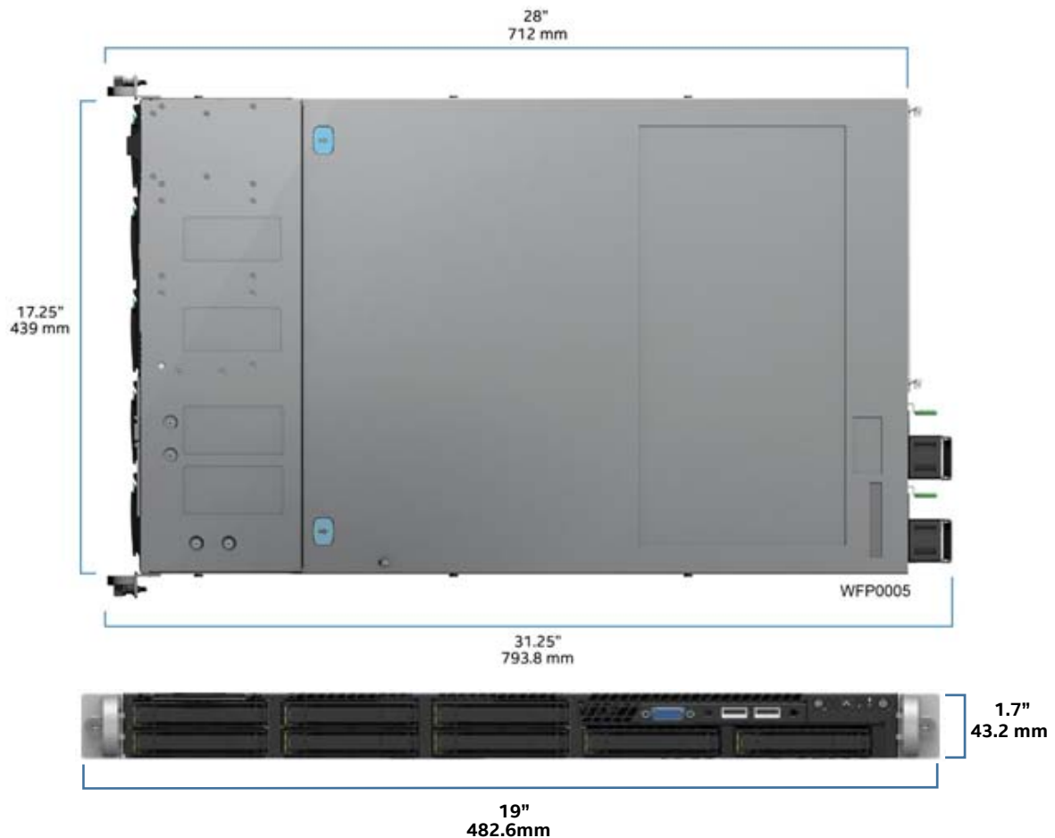
Figure 13. Chassis Dimensions
