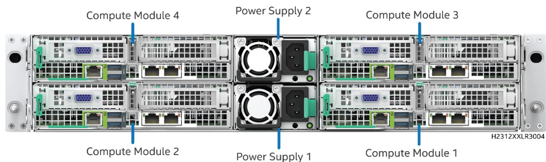
Figure 9. Intel® Server Chassis H2000P family back panel
