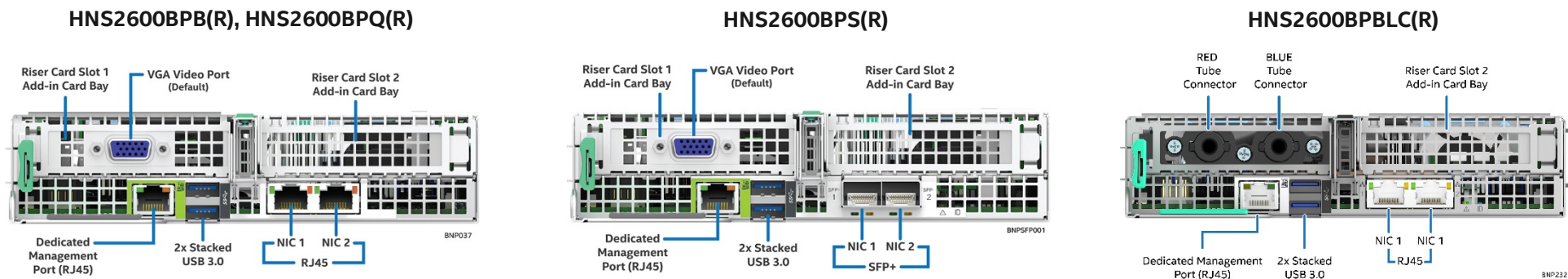
Figure 5. Intel® Compute Module HNS2600BP product family rear connectors
